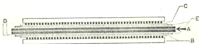
Figure 2. The pyrolysis unit: A, stainless steel tube, 0.006 in. i.d.; B, Fiberglass insulation; C, heating wire; D, thermocouple; E, outer tubing.
